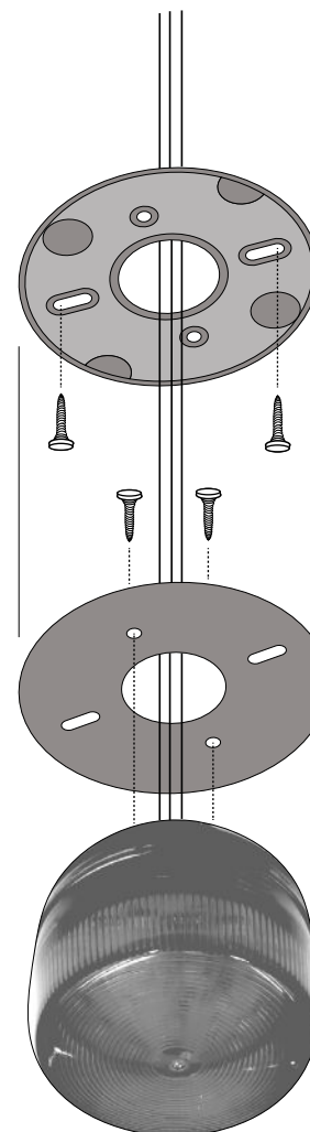
Mounting Bracket 1
