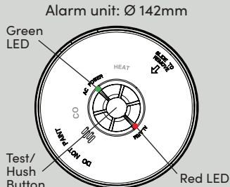
FIG.2 Front View
