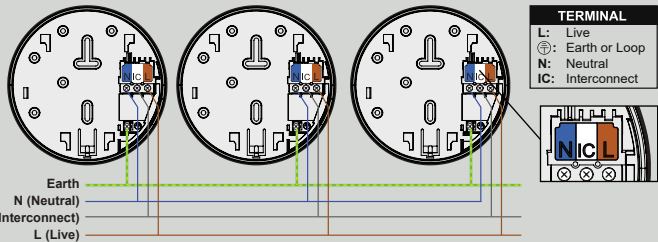
FIG.11 Interconnecting Fire Alarms
