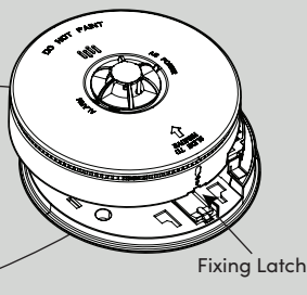
FIG.6 Positioning the smoke/heat detector
