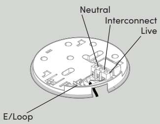
FIG.10 Back View
