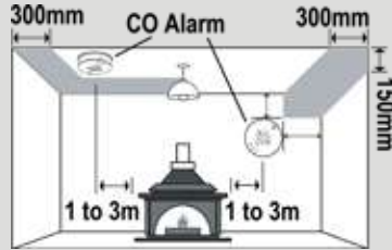
FIG.6.1 Position of the alarm in a room with fuel burning appliance room with fuel burning appliance
