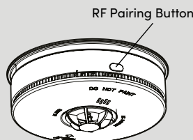
FIG.4 Installed View
