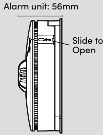
FIG.3 Side View
