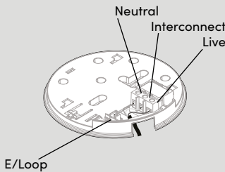
FIG.8 Back View
