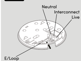
FIG.8 Back View
