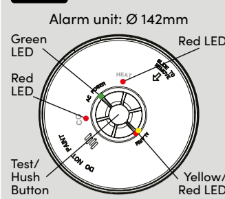
FIG.2 Front View
