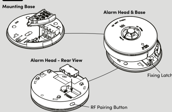
FIG.5 Installed View
