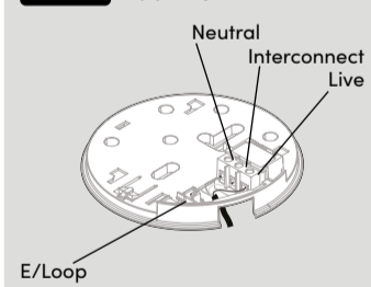
FIG.10 Back View
