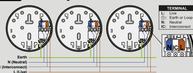
FIG.11 Interconnecting Fire Alarms
