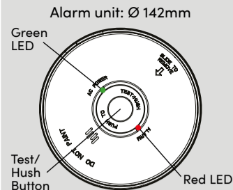
FIG.2 Front View
