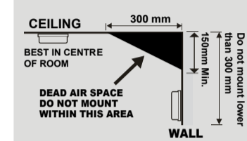
FIG.6 Positioning the smoke/heat detector
