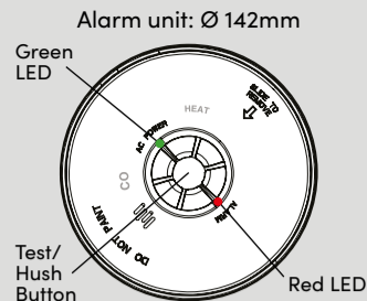
FIG.2 Front View
