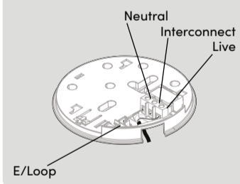
FIG.10 Back View
