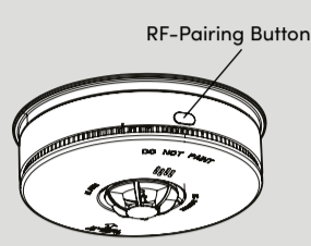
FIG.4 Installed View
