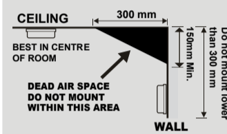
FIG.6 Positioning the smoke/heat detector
