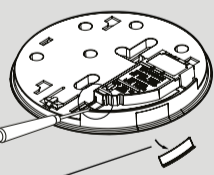
FIG.9 Lift the terminal cover out from the mounting base
