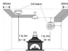
FIGURE 1 - POSITION OF ALARM IN A ROOM WITH FUEL BURNING APPLIANCE
