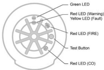
Figure 9 – Alarm indication
