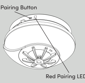
FIG.4 Installed View
