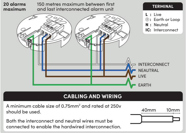
FIG.10 Interconnecting Heat Alarms
