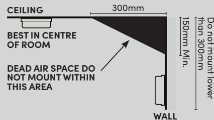
FIG.6 Positioning the Smoke/Heat Alarm
