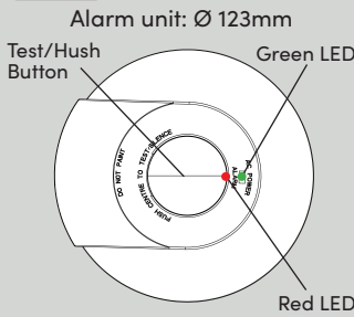
FIG.2 Front View
