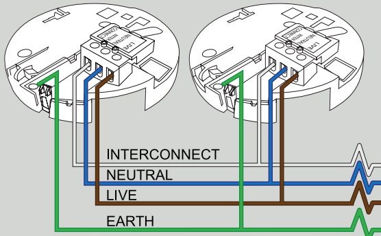
FIG.10 Interconnecting Fire Alarms
