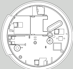
FIG.1 Back View
