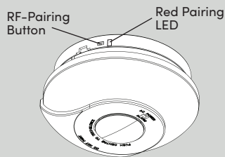
FIG.4 Installed View
