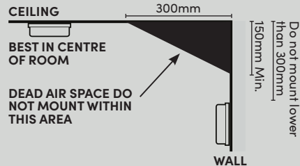
FIG.6 Positioning the Smoke/Heat Alarm
