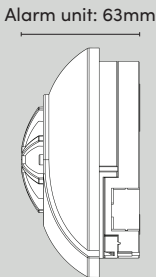
FIG.3 Side View
