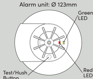
FIG.2 Front View
