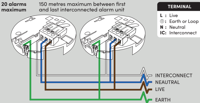
FIG.10 Interconnecting Heat Alarms
