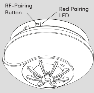
Fig.4 Installed View
