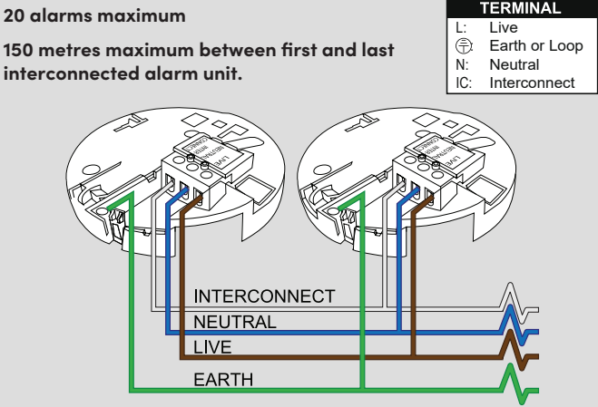
Fig.8 Interconnecting Fire/CO Alarms
