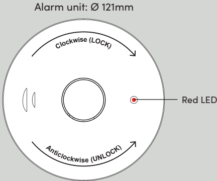
FIG.4 Installed View
