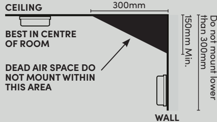
FIG.5 Positioning the Smoke/Heat Alarm
