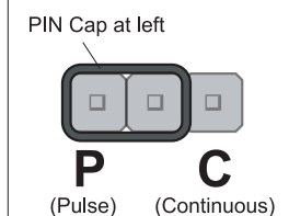
Alternative Setting: Pulse Operation
