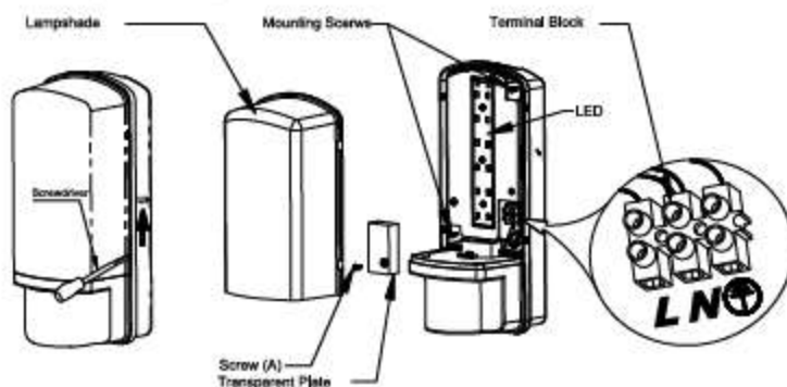
Mounting and Wiring to Terminal
